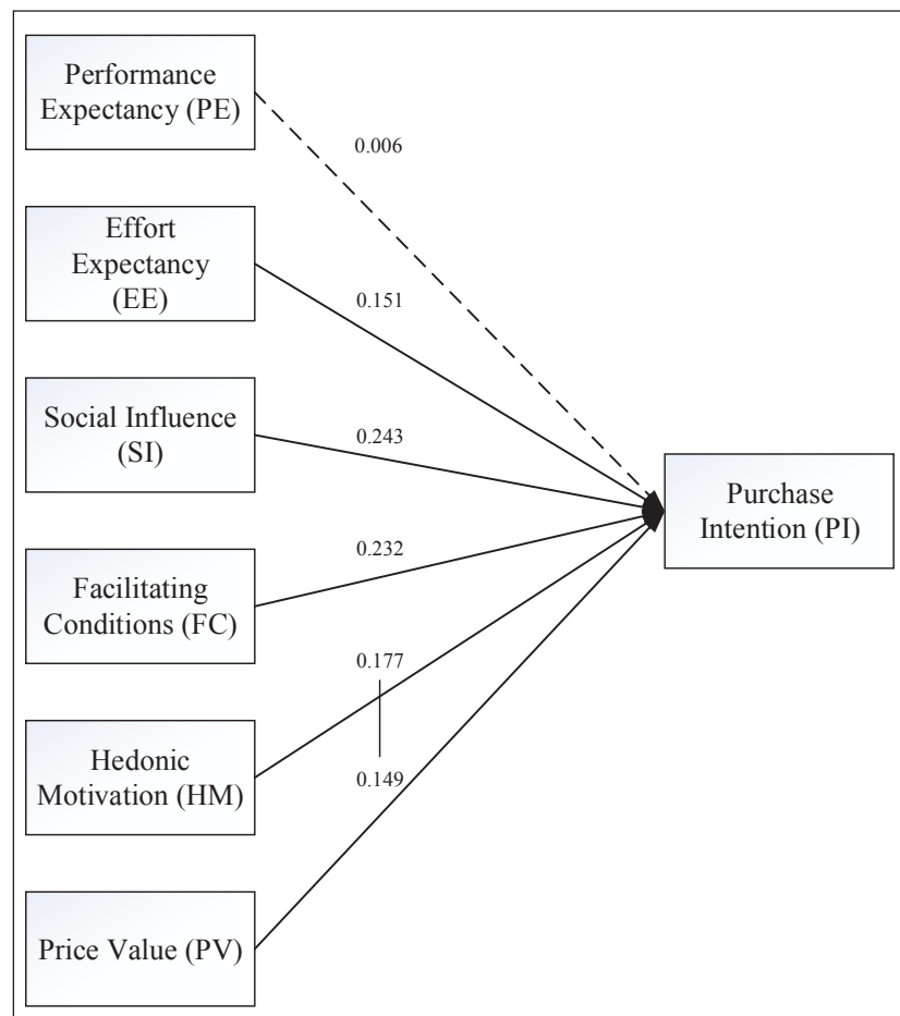
Fig. 3: Model Evaluation Results
