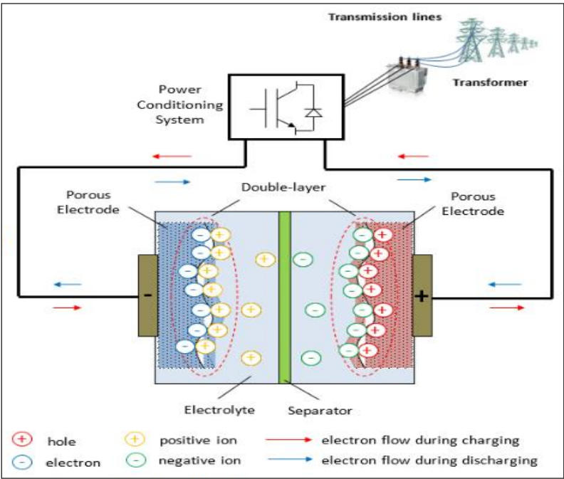
Fig. 2: A Schematic Diagram of a Supercapacitor at the Charged State
