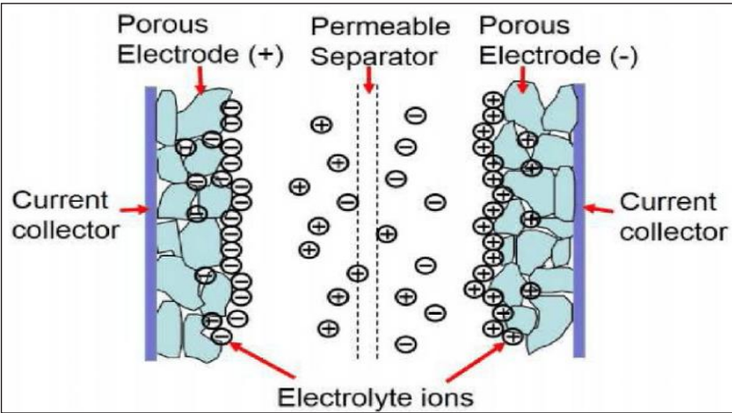
Fig. 2: A Schematic Diagram of a Supercapacitor at the Charged State
