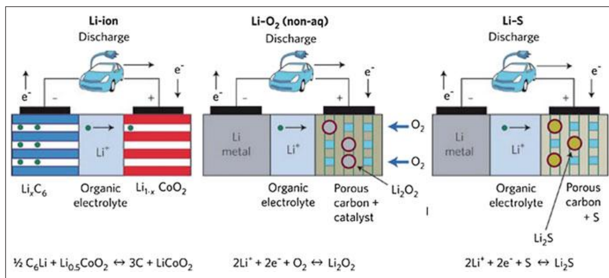
Fig. 3: Schematic Representation of Li-Ion, Non-Aqueous Li-O 2 , and Li-S Batteries [29] Copyright 2016 Royal Society of Chemistry
