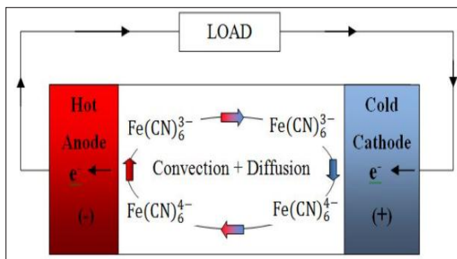
Fig. 4: Ferro-/Ferricyanide Redox Thermogalvanic Cell [36] Copyright by 2012 Springer
