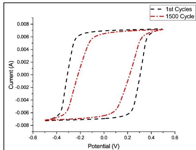
Fig. 4: Life Cycle Test for Fabricated Supercapacitor
