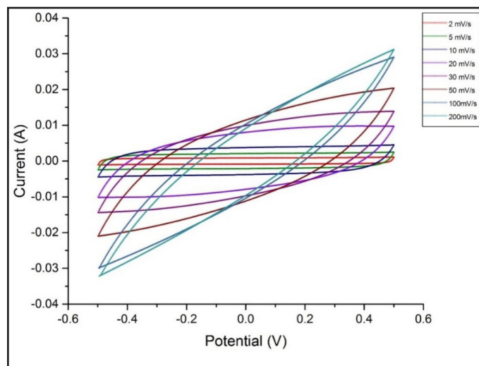
Fig. 3: Cyclic Voltammetry Measurements at Different Scan Rates
