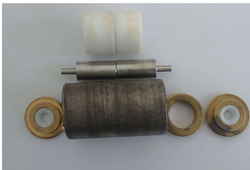
Fig. 1: Completed Newly Designed Test Cell with its Parts
