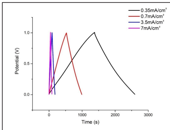
Fig. 6: Charge-Discharge Measurements for Different Current Densities
