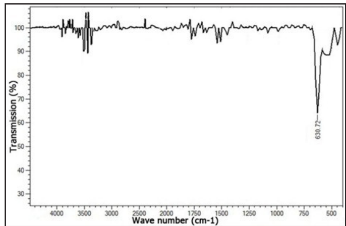
Fig. 3: Shows the FTIR Spectrum of Surface of Cu 2 O layer
