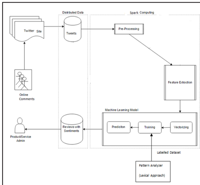
Fig 1: Architecture of Twitter Sentiment Analysis using Apache Spark and Combination of Lexical and Machine Learning Technique
