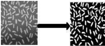
Fig 4: Thresholding Process
