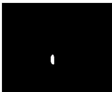
Fig 5: : Regionprops example
