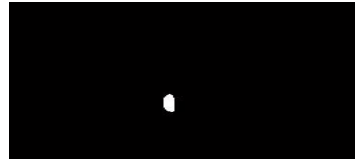
Fig 5: Regionprops example
