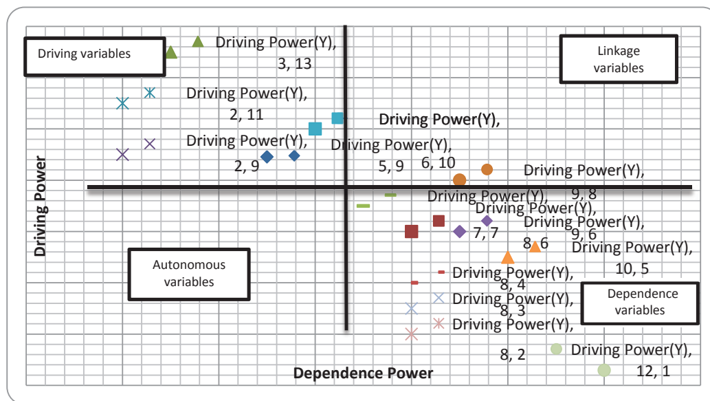
Fig. 5: MICMAC analysis
