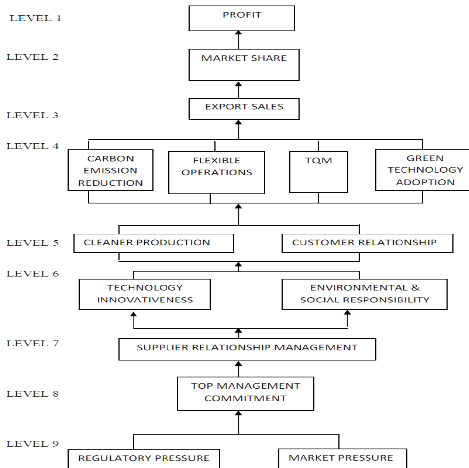
Fig. 4: ISM Model
